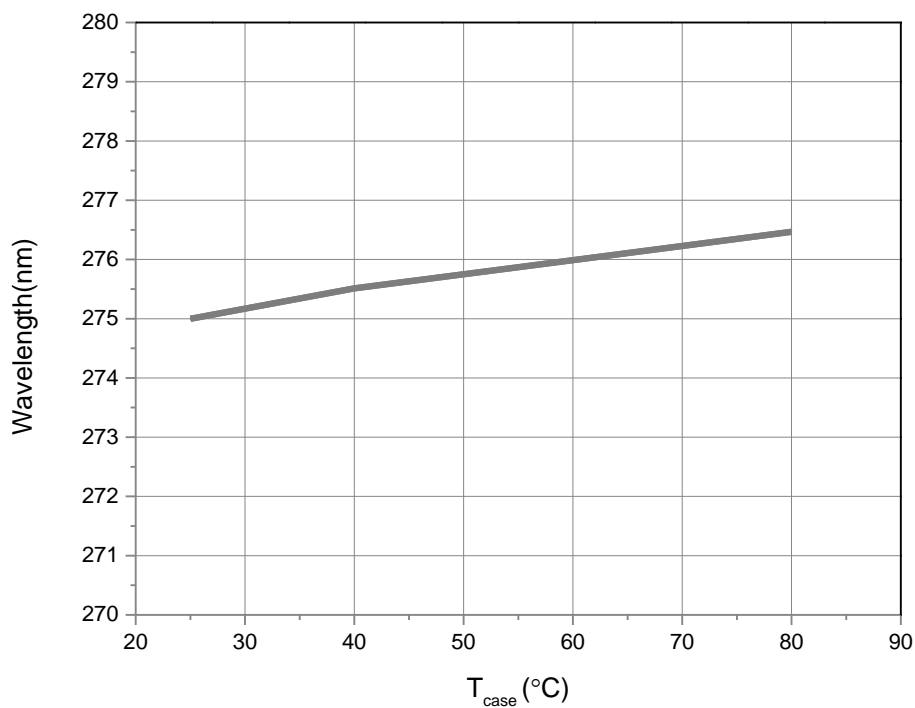
Fig 6. Peak Wavelength vs. Case Temperature, I_F=20\text{mA}
